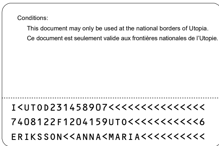
Figure A-4. Reverse side of a TD1 Size MROTD showing the MRZ and including a condition in Zone VI, the Optional Document Data Element zone
